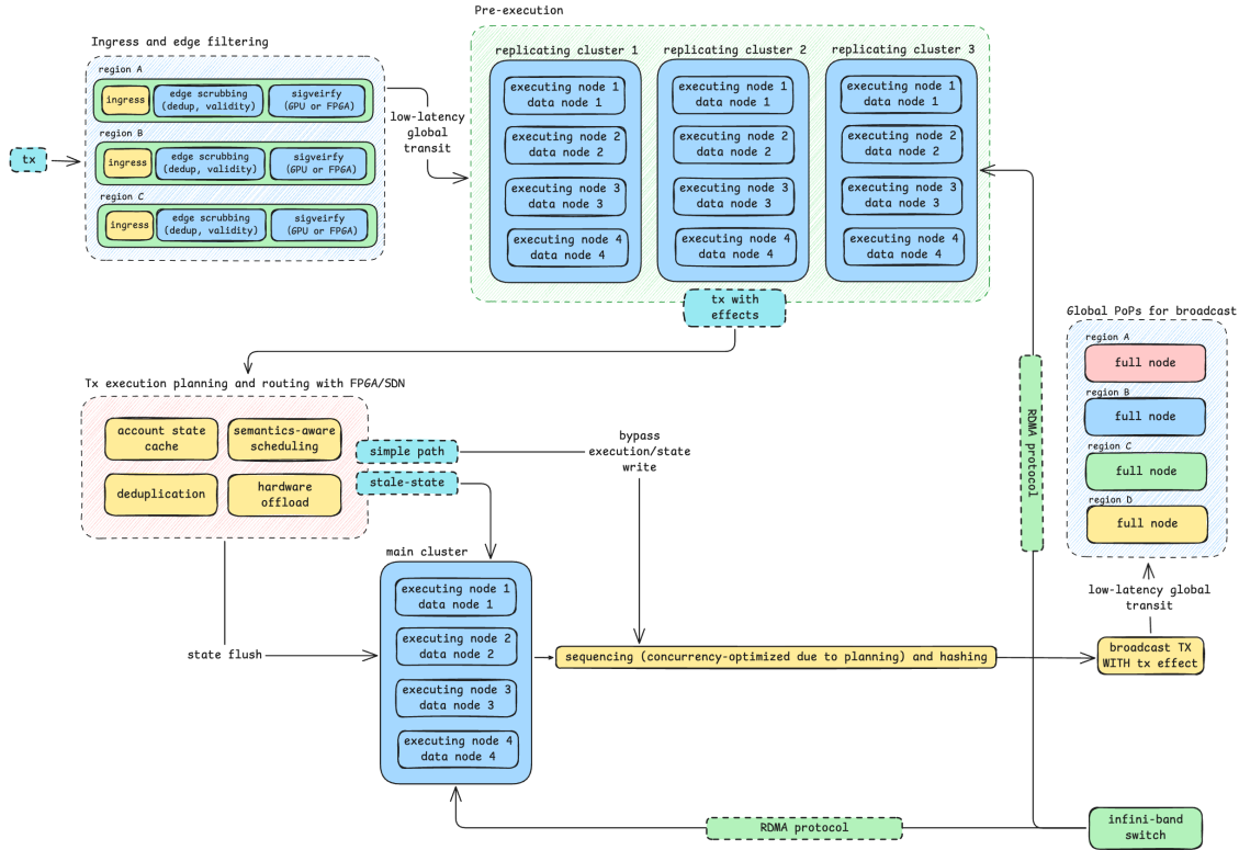
Figure 1: System architecture
